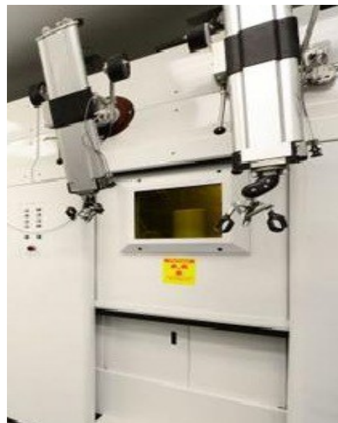
Figure F-1 Example of a hot cell with remote manipulators
